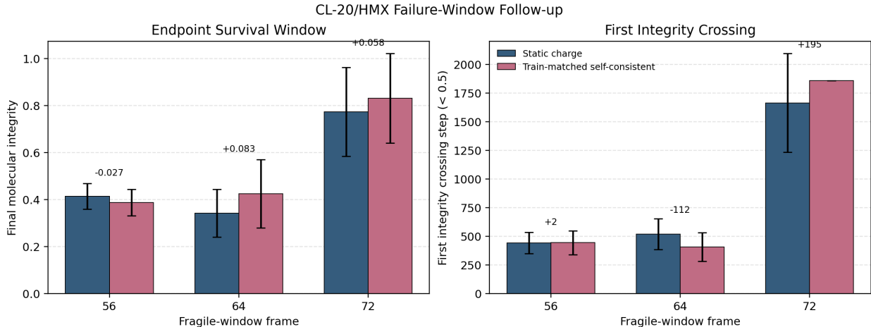
Figure 7: Dense CL-20/HMX fragile-window follow-up comparing static_charge against train-matched self_consistent . The positive dynamic signal is not a broad onset advantage. Instead, endpoint survival improves only in a narrow local window: frame 56 remains unfavorable, frame 64 shows a modest final-integrity gain, and frame 72 shows the clearest combined endpoint benefit.
