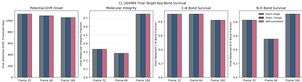
Figure 6: CL-20/HMX final-target focused key-bond survival rerun on the most sensitive frames 32, 64, and 160. Potential-drift onset, molecular integrity, and C–N / N–O bond-family survival all vary substantially across starting frames, but remain nearly unchanged across the three model families within each frame.
