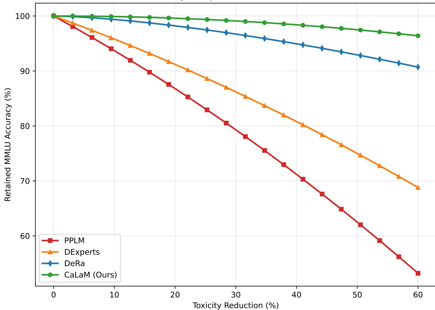
RealToxicityPrompts Frontier (34B Backbone)
