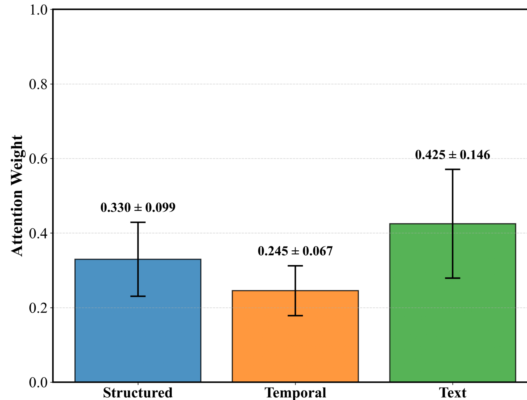
Modality Contribution Analysis
