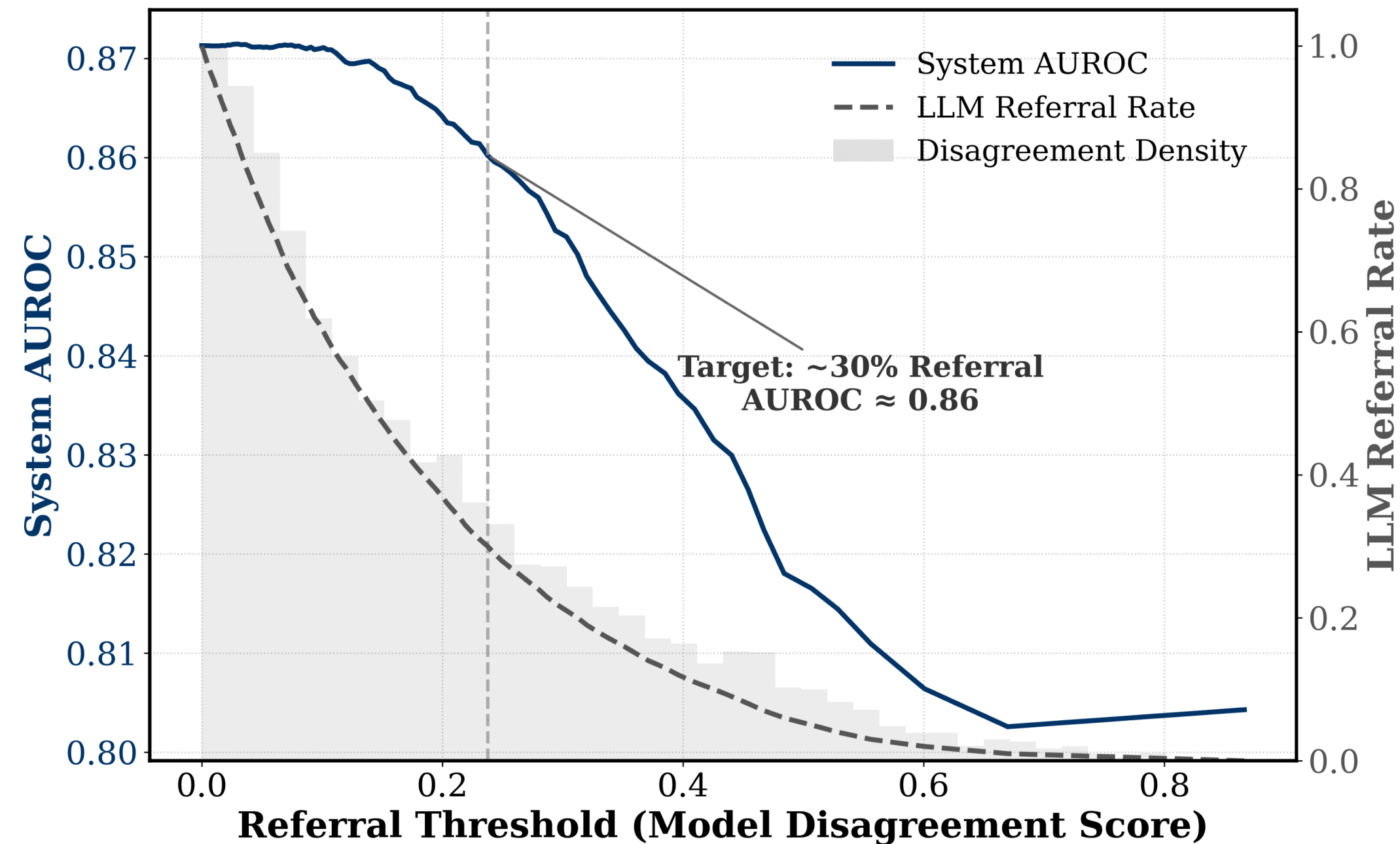
Performance-Cost Trade-off Analysis
