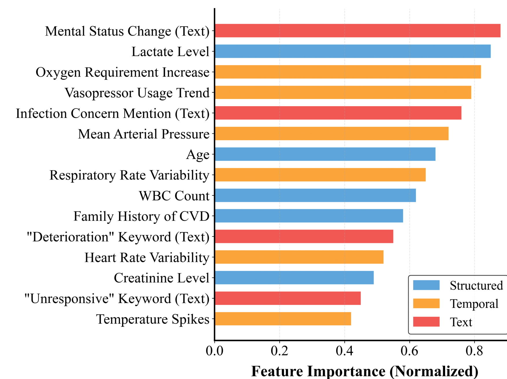
Global Feature Importance Analysis
