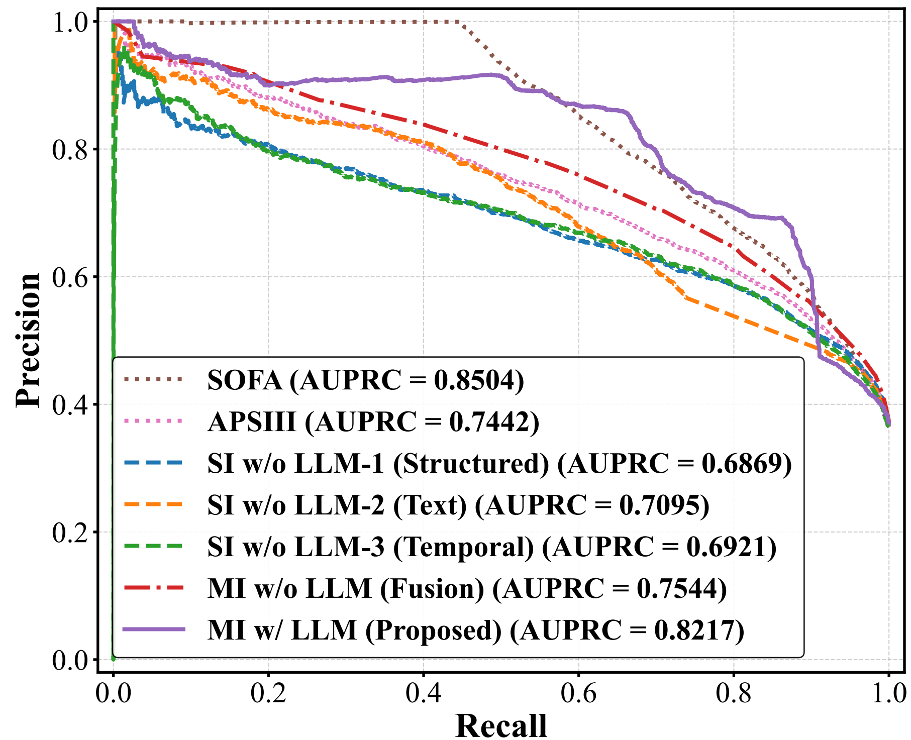
Precision-Recall Curve (PRC)
