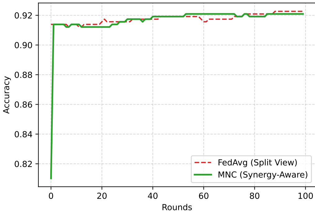
Standard Benchmark: Breast Cancer VFL (Sklearn)
