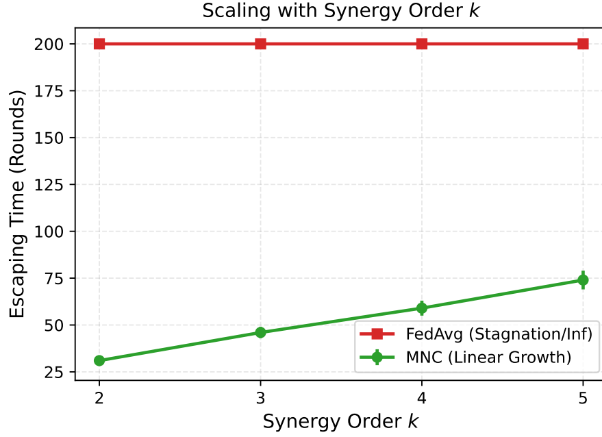
Figure 4. Escaping Time vs Synergy Order k . MNC scales linearly while standard FL methods remain stagnant indefinitely.
