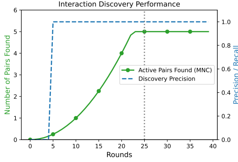
Figure 1. Discovery Performance. MNC Pursuit recovers all active interaction pairs within 25 rounds with zero false discovery after the noise threshold is crossed.
