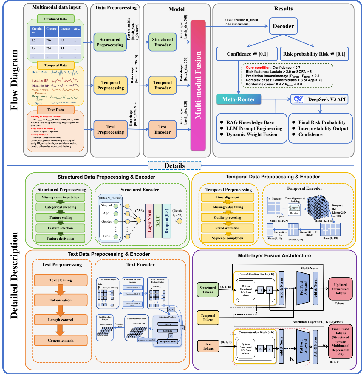
Figure 2: Overall architecture of Cardio-Hybrid Net, including tri-stream encoders, cross-modal attention, uncertainty estimation, and LLM routing.
