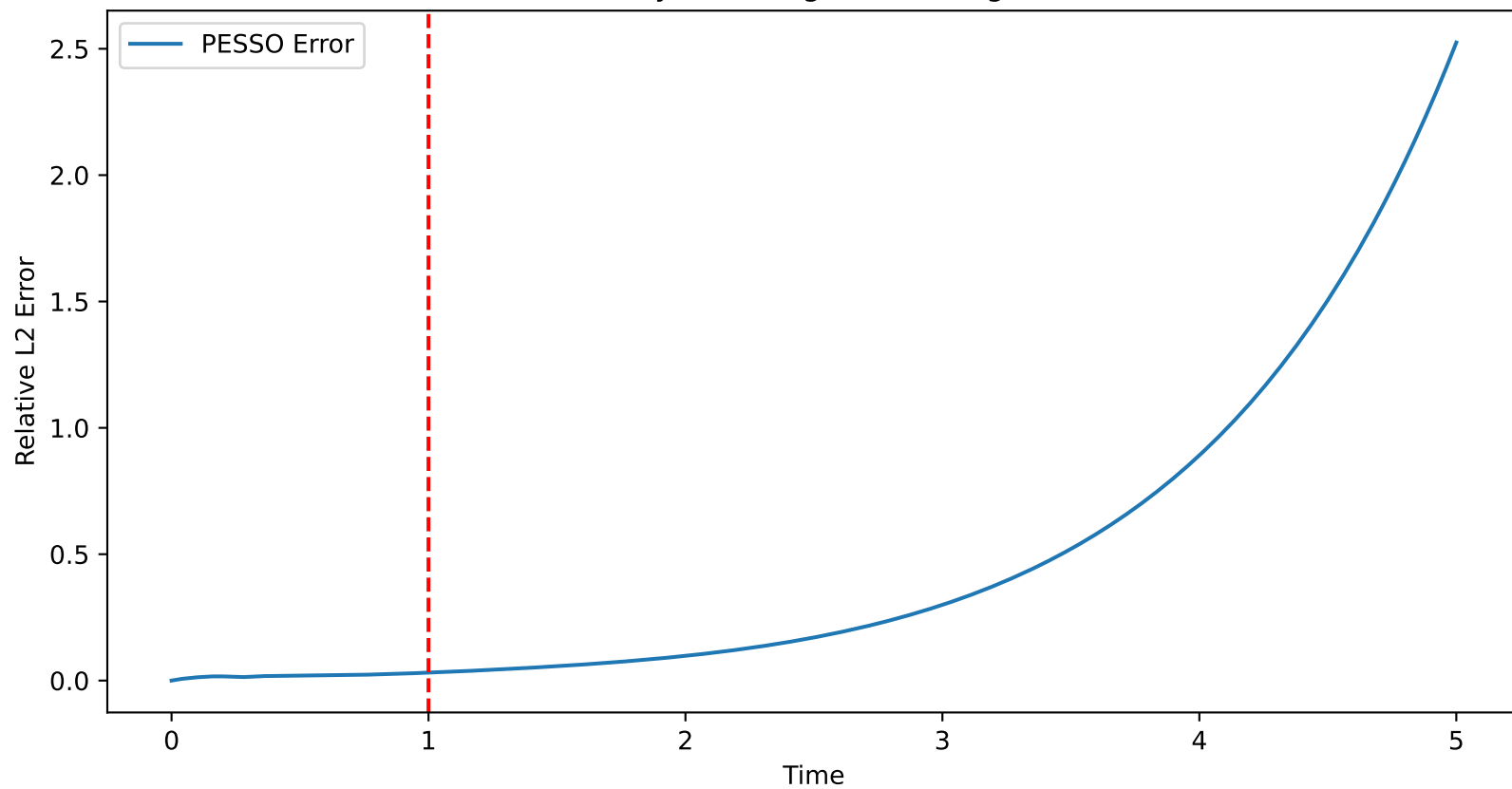
Quality Cliff Diagnostic (Burgers)
