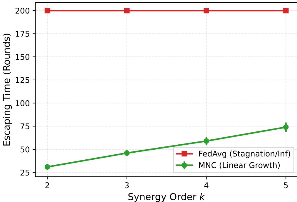
Scaling with Synergy Order k
