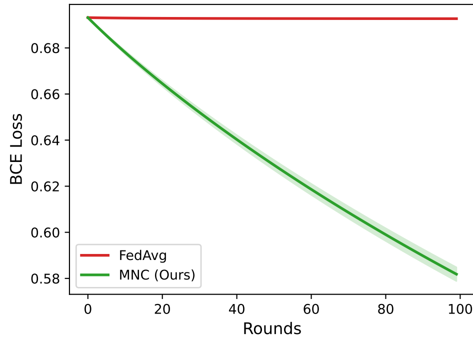
Training Loss
