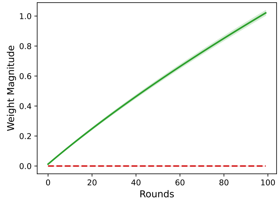
Interaction Energy |\theta_{12}|
