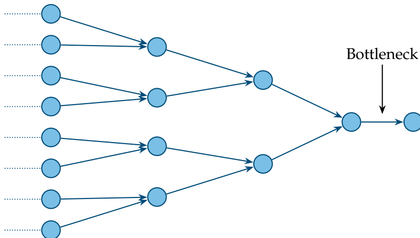
Figure 8.2: The receptive field of a node, unrolled over layers, typically grows exponentially: each additional hop multiplies the number of nodes that must be summarized. The representation gathering this region is a vector of fixed size, independent of how many nodes feed into it, so information from the wider neighborhood is compressed, reducing the contribution of any single distant node.
