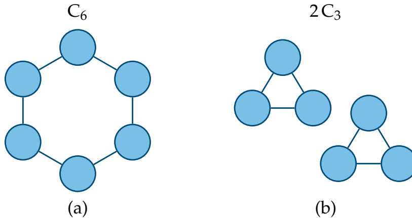
Figure 8.3: Two non-isomorphic regular graphs in which every node has the same degree. The 1-WL test colors all nodes of both graphs identically and never separates them, so no message-passing network can tell the two graphs apart, although they are not isomorphic.
