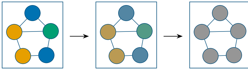
Figure 8.1: Node representations at increasing depth. With few layers the representations of different nodes remain distinct; as layers are stacked, repeated smoothing drives them together, until at large depth the nodes of each connected component converge toward a common representation and can no longer be told apart.
