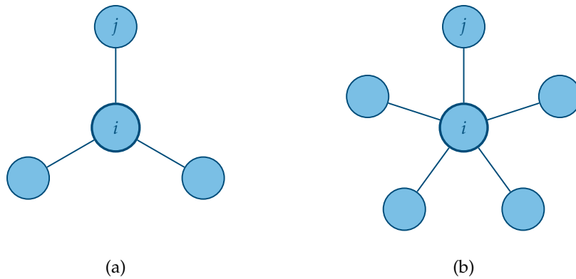
Figure 4.2: Two nodes with neighborhoods of different sizes: the node on the left has three neighbors, the node on the right has five. A model that processes a node together with its neighbors must accept inputs of varying size, which a multilayer perceptron cannot.
