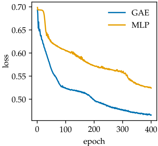
training
