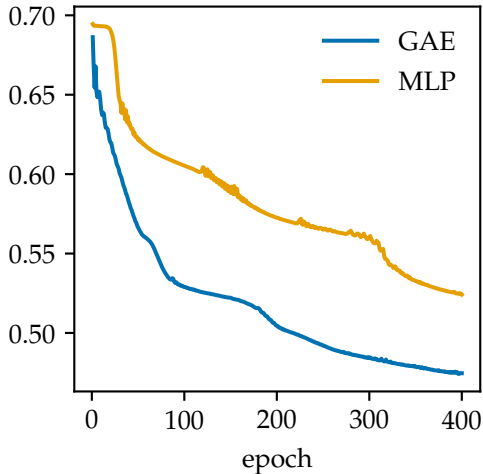
validation
