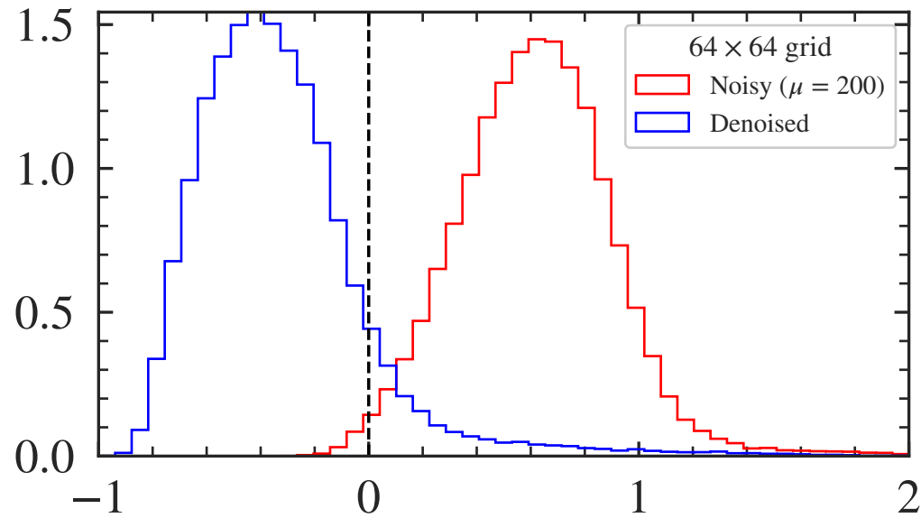
(b) p_T response
