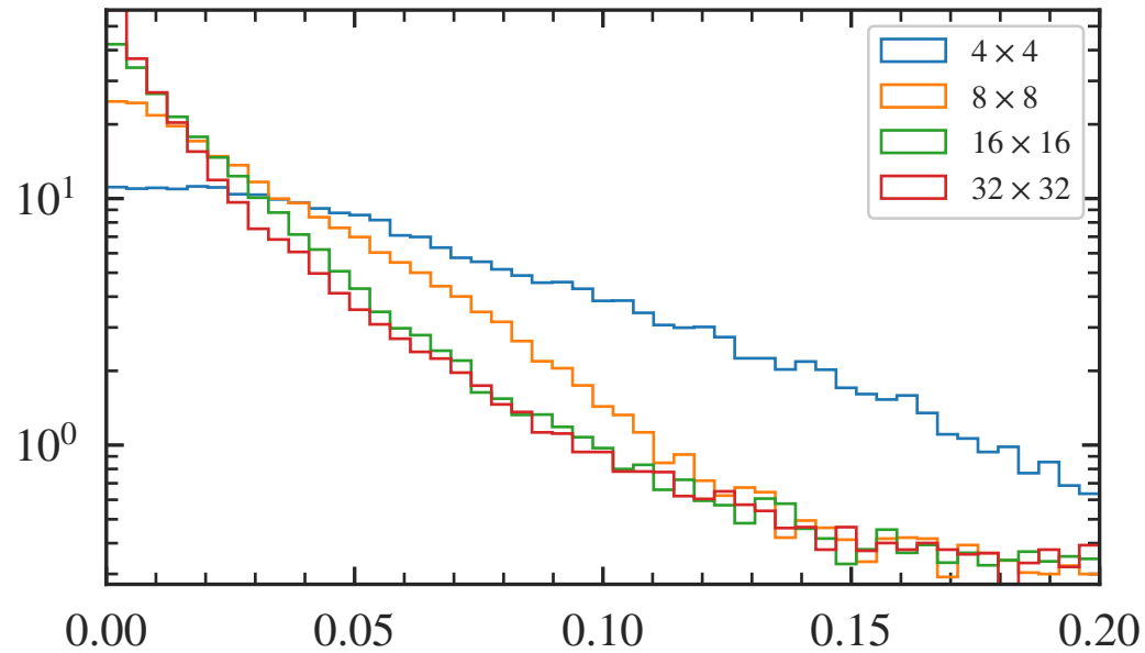
(b) p_T relative resolution
