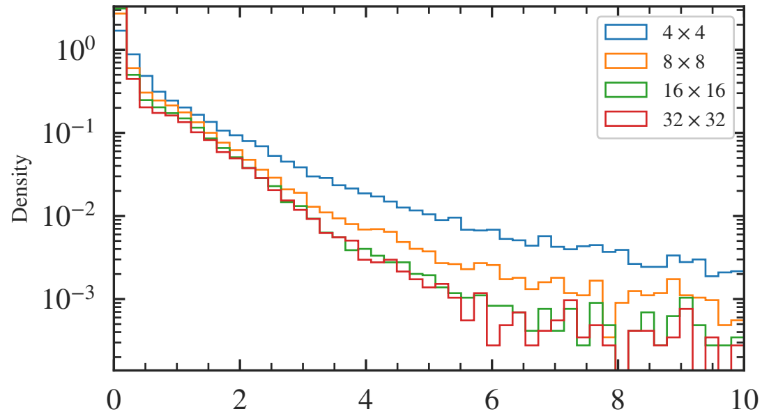
(a) mass relative resolution
