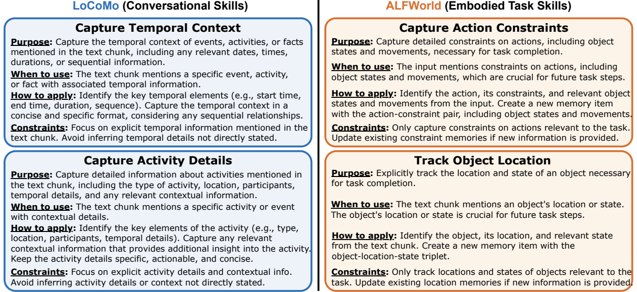
Figure 4. Case study. We show representative evolved skills learned on LoCoMo and ALFWorld.
