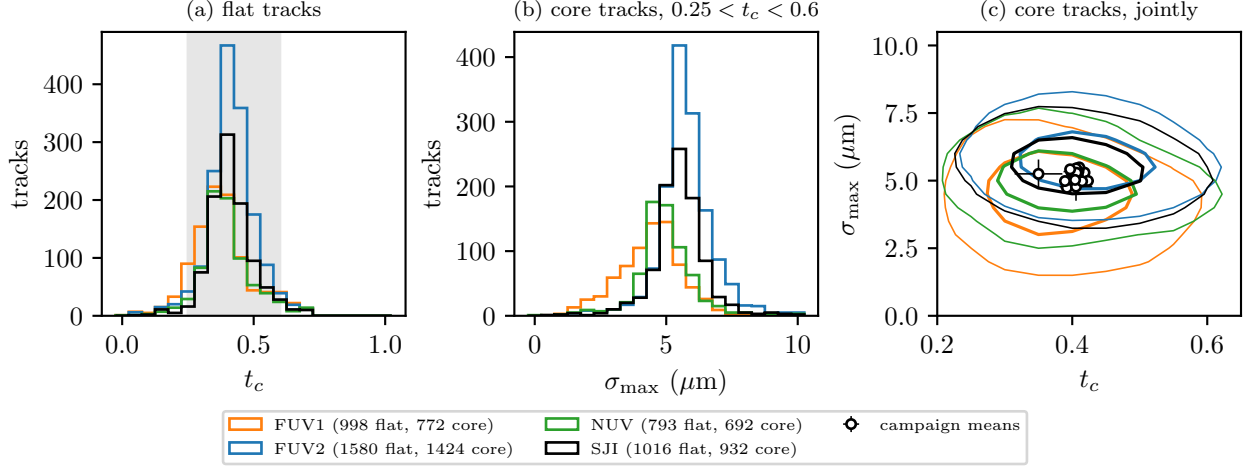
Fig 6 The fitted parameters. (a) The critical depth of every flat track on each CCD. The tails below 0.25 and above 0.6 are tracks Equation 1 describes poorly, sharp or diffuse along most of their length, and they are excluded from the shaded core used elsewhere. (b) The back-surface width of the core tracks. (c) The joint distribution of the core tracks on each CCD, as the contours enclosing half (thick) and nine tenths (thin) of them, on the grid the fits are searched over (0.05 in t_c and 0.5 \mu\text{m} in \sigma_{\text{max}} ) smoothed by one cell, with the mean of each campaign of Table 1 and its standard error as an open circle. The campaigns, spanning two particle populations, four spacecraft rolls, and the spectrograph and slit-jaw CCDs, agree to within a few hundredths in t_c , and the contours run wider in \sigma_{\text{max}} than in t_c , since a single track constrains its back-surface width less well than the depth at which it sharpens.
