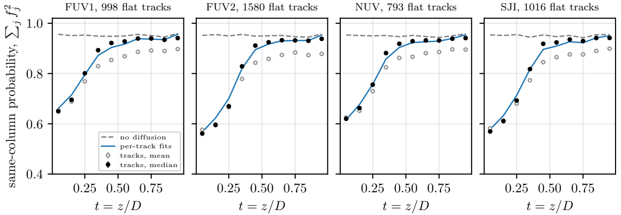
Fig 7 The probability that two electrons deposited in the same slice are collected in the same column, over the flat tracks on each CCD in bins of fractional depth. The dashed line is Equation 1 with no charge diffusion, averaged over the slices of each bin, which is below one only where a centerline runs near a pixel boundary, and the blue line is the same at each track's own fit. The black points are the dashed line minus the median, over the slices of the bin, of how far each slice falls short of its own no-diffusion value, with the standard error of the median; the open points are the plain mean of the slices. Charge from other hits in the frame that touched a track and was cut out with it can only lower the sum, so the mean sits below the median wherever such charge is common, beyond t_c on all four CCDs, while at the back surface the two agree. The back surface is lowest on the FUV2 and SJI CCDs and highest on FUV1.
