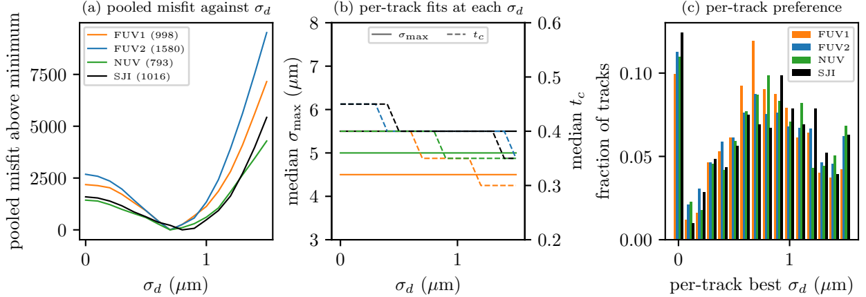
Fig 5 The spread inside the depletion region, \sigma_d in Equation 1, which is shared by every track on a CCD. (a) The misfit summed over the flat tracks on each CCD at each \sigma_d , with each track refit in t_c , \sigma_{\max} , orientation, and centerline, shown relative to its minimum, which lies at \sigma_d = 0.70 \mu\text{m} on FUV1, 0.70 \mu\text{m} on FUV2, 0.70 \mu\text{m} on NUV, and 0.80 \mu\text{m} on SJI. (b) The median t_c and \sigma_{\max} of the same tracks at each \sigma_d : the spread inside the depletion region trades against the field-free wedge, stepping t_c down while \sigma_{\max} holds. (c) The \sigma_d each flat track prefers on its own. The preference of any one track is weak, spread over the whole grid, and it is only in the sum that the minimum is sharp.
