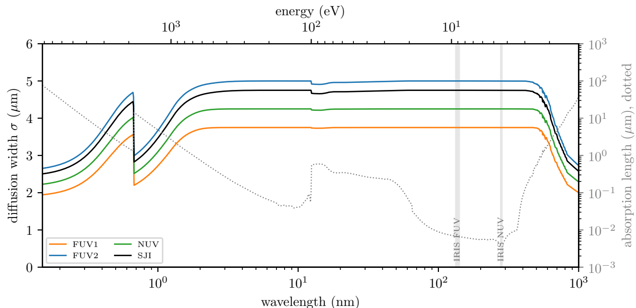
Fig 8 The width of the charge cloud a photon leaves in each CCD, against the wavelength of the photon. The width is the standard deviation of the cloud. A photon is absorbed at a random depth, exponentially distributed with the absorption length of silicon (dotted, from the tabulated optical constants 12,13 ), and the charge it liberates spreads by the width measured at that depth in Figure 4b, held at the value of its first bin up to the back surface. The curve is the standard deviation of the cloud that results, which is the square root of the squared width averaged over depth, weighted by the fraction of photons absorbed at each depth; photons that pass through the 14 \mu\text{m} of silicon are not counted. Between 30 and 350 nm every photon is absorbed within 10 nm of the back surface, and the cloud has the back-surface width of Table 2. In the visible and in the soft X-rays the photons penetrate to the depletion region and the cloud narrows. Near the band gap silicon is nearly transparent, and the few photons absorbed are spread through its thickness.
