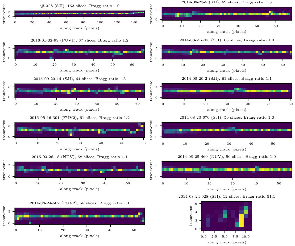
Fig 9 The eleven longest flat tracks and, in the last panel, the track with the strongest Bragg rise, as the finder cut them out: seven pixels wide, re-centered on the integer part of the fitted centerline in every slice, and oriented with the back surface at the left. Each panel’s color scale is clipped at its 98th percentile so that a single bright pixel does not hide the track. The stopping track’s charge per slice climbs by a factor of twenty toward one end, and the selection of Section 2 rejects it.
