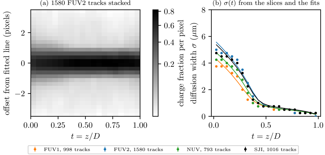
Fig 4 (a) Every slice of every flat track on the FUV2 CCD placed at its fractional depth and aligned on its fitted centerline, with each pixel's charge spread uniformly over its own width. The wedge is subtle: the wings at t < 0.4 carry a few percent of the charge. (b) Points: the diffusion width in each depth bin on each CCD, found by summing the misfit of every slice in the bin over a grid of trial widths and minimizing, with no parametric model of the depth dependence; the error bars span the widths within two units of misfit of the minimum. Lines: the average of the per-track fits of Equation 1 on the same CCD, which reproduces the model-free profile at every depth, including the floor of a few tenths of a micron beyond t_c that the \sigma_d term supplies.
