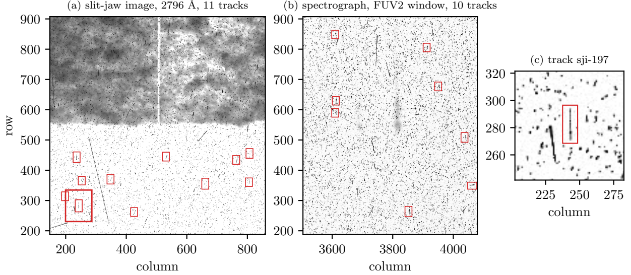
Fig 1 Level-1 images taken seconds apart during a pass through SAA on 2018 May 4, frames 39498499 and 39498504, with the spacecraft rolled by -90^\circ so that the limb runs horizontally across the field. (a) The slit-jaw image at 2796 Å, whose lower half is off the limb. (b) The widest of the readout windows of the spectrograph image, on the FUV2 CCD. (c) One of the tracks in (a) at full resolution. The images are shown with an inverse hyperbolic sine stretch above the background, saturating at 400 data numbers, and the red boxes outline the tracks the finder kept from each frame. Most of the particle hits are the short streaks and dots that pepper both images; the tracks used here are the long, thin, nearly vertical ones.
