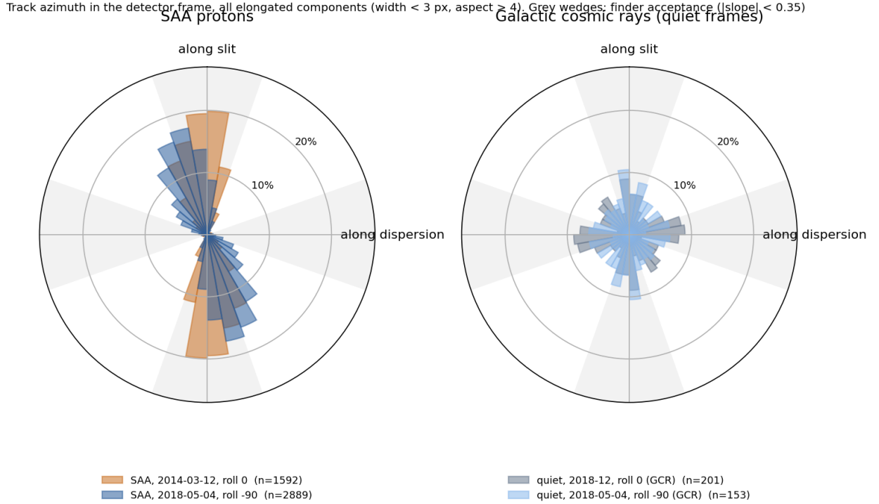
Fig 2 The azimuth in the detector frame of every elongated connected component above 5\sigma in the spectrograph frames, with a charge-weighted width under 3 pixels and an aspect ratio over 4, before any of the finder's cuts, so that the whole circle is populated. Tracks are undirected, so each is drawn at \theta and \theta + 180^\circ , and the grey wedges are the windows about the row and column axes that the finder accepts. Left: the frames taken inside SAA at both spacecraft rolls. Right: quiet frames at the same rolls. The trapped protons arrive strongly aligned, mostly within the window along the slit, while the cosmic rays are isotropic to within counting noise; the preferred direction shifts and broadens when the spacecraft is rolled, so it is a property of the arrival direction as seen by the instrument rather than of the detector.
