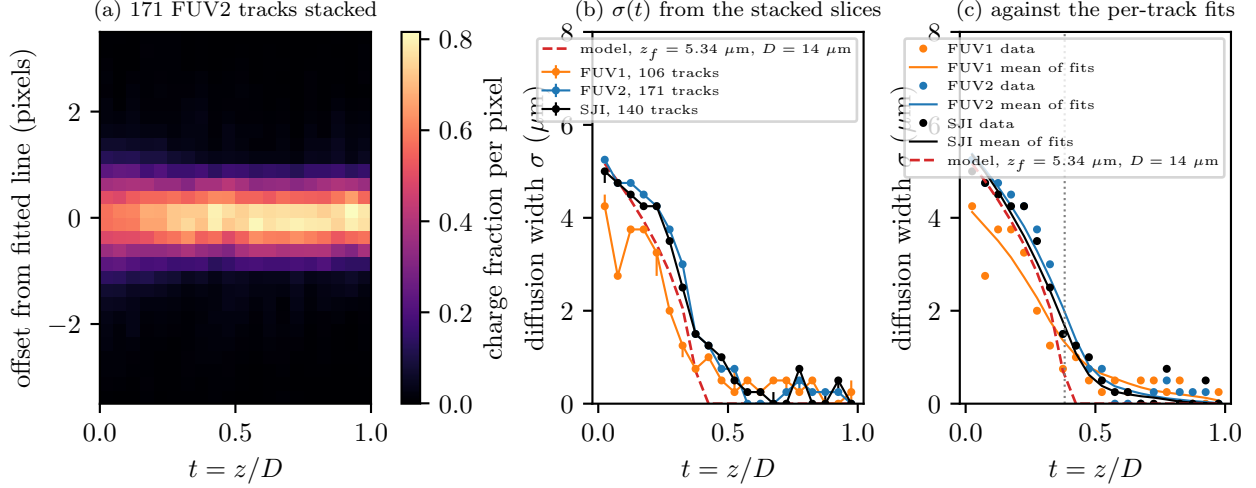
Fig 4 (a) Every slice of every flat track on the FUV2 CCD placed at its fractional depth and aligned on its fitted centerline, with each pixel's charge spread uniformly over its own width. The wedge is subtle: the wings at t < 0.4 carry a few percent of the charge. (b) The diffusion width in each depth bin, found by summing the misfit of every slice in the bin over a grid of trial widths and minimizing, with no parametric model of the depth dependence. Error bars span the widths within two units of misfit of the minimum. (c) The same points against the average of the per-track fits of Equation 1, which reproduces the model-free profile except beyond t_c , where the tracks keep a floor of 0.5 to 1 \mu\text{m} that the model sets to zero.
