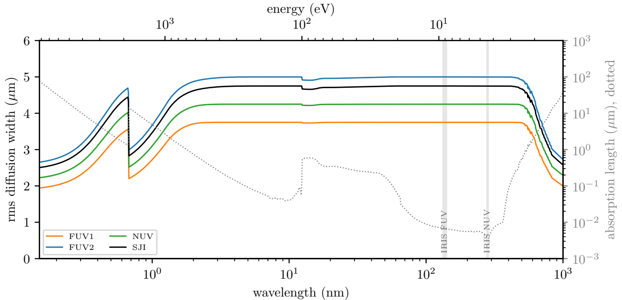
Fig 8 The measurement as an instrument designer needs it: the width of the charge cloud of a photon against its wavelength, from soft X-rays to the band gap of silicon. A photon is absorbed at a depth drawn from the exponential with the absorption length of silicon (dotted, from the tabulated optical constants 12,13 ), among the photons absorbed within the 14 \mu\text{m} thickness, and the root mean square of the model-free width of Figure 4b, held at the value of its first bin up to the back surface, is taken over that depth. From 30 to 350 nm the absorption length is under 10 nm, so the whole ultraviolet sees the back-surface width of Table 2; through the visible, and again in the soft X-rays, the photons reach the depletion region and the cloud narrows; and near the band gap the sensor is nearly transparent and the few photons absorbed are spread through its thickness.
