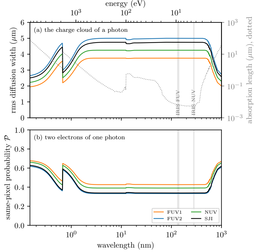
Fig 8 The measurement as an instrument designer meets it, against the wavelength of the photon from soft X-rays to the band gap of silicon. A photon is absorbed at a depth drawn from the exponential with the absorption length of silicon (dotted, from the tabulated optical constants 12,13 ), among the photons absorbed within the 14\ \mu\text{m} thickness, and the measured profiles are averaged over that depth. (a) The root mean square of the model-free width of Figure 4b. (b) The square of the same-column probability of Figure 7, the probability that two electrons of the same photon are collected in the same 13\ \mu\text{m} pixel, which enters the variance of the image. Each profile is held at the value of its first bin up to the back surface. From 30 to 350 nm the absorption length is under 10 nm, so the whole ultraviolet sees the back-surface values of Table 2; through the visible, and again in the soft X-rays, the photons reach the depletion region and the cloud narrows; and near the band gap the sensor is nearly transparent and the few photons absorbed are spread through its thickness.
