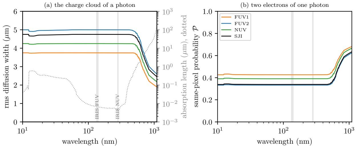
Fig 8 The measurement as an instrument designer meets it, against the wavelength of the photon. A photon is absorbed at a depth drawn from the exponential with the absorption length of silicon (dotted, from the tabulated optical constants 12,13 ), among the photons absorbed within the 14 \mu\text{m} thickness, and the measured profiles are averaged over that depth. (a) The root mean square of the model-free width of Figure 4b. (b) The square of the same-column probability of Figure 7, the probability that two electrons of the same photon are collected in the same 13 \mu\text{m} pixel, which enters the variance of the image. Each profile is held at the value of its first bin up to the back surface. Below 350 nm the absorption length is under 10 nm, so the whole ultraviolet sees the back-surface values of Table 2; through the visible the photons reach the depletion region and the cloud narrows; and near the band gap the sensor is nearly transparent and the few photons absorbed are spread through its thickness.
