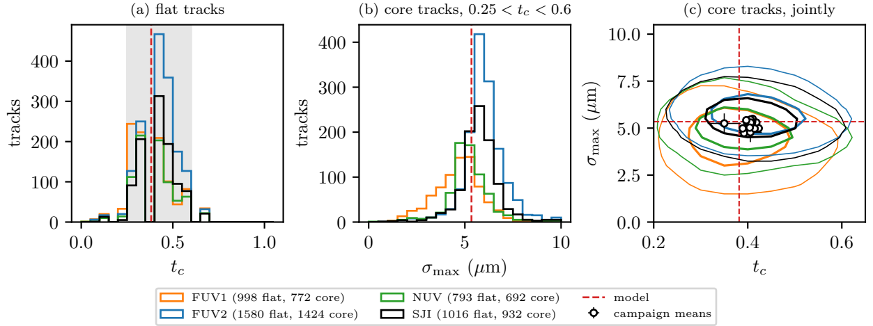
Fig 6 The fitted parameters. (a) The critical depth of every flat track on each CCD, with the field-free model dashed. The tails below 0.25 and above 0.6 are tracks the model describes poorly, sharp or diffuse along most of their length, and they are excluded from the shaded core used elsewhere. (b) The back-surface width of the core tracks. (c) The joint distribution of the core tracks on each CCD, as the contours enclosing half (thick) and nine tenths (thin) of them, on the grid the fits are searched over ( 0.05 in t_c and 0.5 \mu\text{m} in \sigma_{\text{max}} ) smoothed by one cell, with the field-free model at the crossing of the dashed lines and the mean of each campaign of Table 1 with its standard error as an open circle. The campaigns, spanning two particle populations, four spacecraft rolls, and three cameras, agree to within a few hundredths in t_c , all within 0.04 of the model, and the contours run wider in \sigma_{\text{max}} than in t_c , since a single track constrains its back-surface width less well than the depth at which it sharpens.
