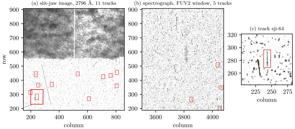
Fig 1 Level-1 images taken seconds apart during a pass through SAA on 2018 May 4, with the spacecraft rolled by -90^\circ so that the limb runs horizontally across the field. (a) The slit-jaw image at 2796 Å, whose lower half is off the limb. (b) The widest of the readout windows of the spectrograph image, on the FUV2 CCD. (c) One of the tracks in (a) at full resolution. The images are shown with an inverse hyperbolic sine stretch above the background, saturating at 400 data numbers, and the red boxes outline the tracks the finder kept from each frame. Most of the particle hits are the short streaks and dots that pepper both images; the tracks used here are the long, thin, nearly vertical ones.
