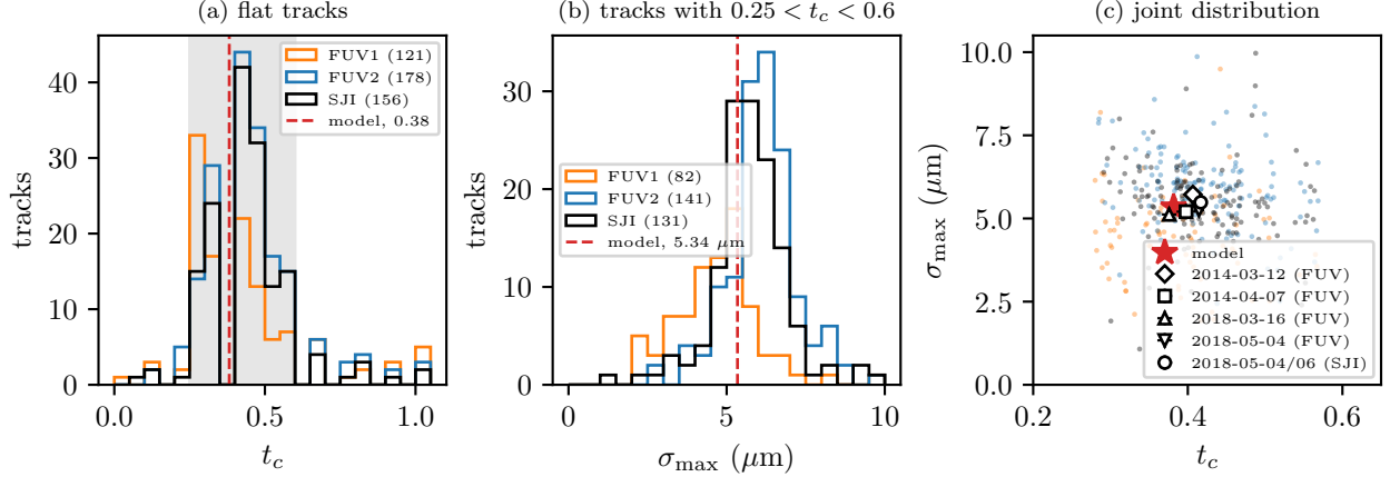
Fig 6 The fitted parameters. (a) The critical depth of every flat track on each CCD, with the field-free model dashed. The pile-up at t_c = 1 and the tail below 0.25 are tracks the model cannot describe, diffuse or sharp along their whole length, and they are excluded from the shaded core used elsewhere. (b) The back-surface width of the core tracks. (c) Each core track jittered off the fit grid, colored by CCD as in (a), with the mean of each dataset and its standard error as open symbols. Two particle populations, two spacecraft rolls, and two cameras agree to within a few hundredths in t_c , all within 0.04 of the model, and the diagonal smear is the degeneracy between t_c and \sigma_{\max} in a single-track fit.
