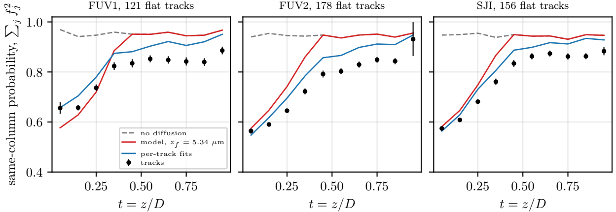
Fig 7 The probability that two electrons deposited in the same slice are collected in the same column, averaged over the flat tracks on each CCD in bins of fractional depth, with the standard error of each mean. The red line is the field-free model, Equation 1 with t_c = 0.38 and \sigma_{\max} = 5.34 \mu\text{m} , evaluated at the fitted centerline of each track and averaged in the same bins; the blue line is the same for each track's own fit; and the dashed line is the same with no charge diffusion, which is below one only where a centerline runs near a pixel boundary. The back surface agrees with the model on the FUV2 and SJI CCDs, while beyond t_c the tracks settle below the no-diffusion curve on all three.
