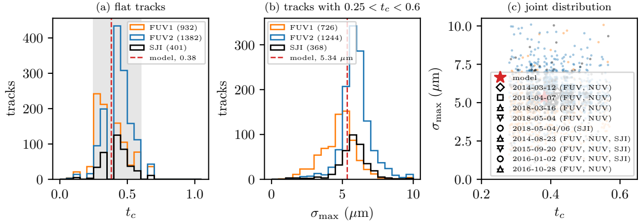
Fig 6 The fitted parameters. (a) The critical depth of every flat track on each CCD, with the field-free model dashed. The tails below 0.25 and above 0.6 are tracks the model describes poorly, sharp or diffuse along most of their length, and they are excluded from the shaded core used elsewhere. (b) The back-surface width of the core tracks. (c) Each core track jittered off the fit grid, colored by CCD as in (a), with the mean of each dataset and its standard error as open symbols. Two particle populations, two spacecraft rolls, and two cameras agree to within a few hundredths in t_c , all within 0.04 of the model, and the diagonal smear is the degeneracy between t_c and \sigma_{\text{max}} in a single-track fit.
