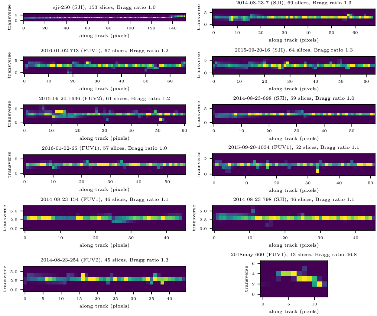
Fig 8 The eleven longest flat tracks and, in the last panel, the track with the strongest Bragg rise, as the finder cut them out: seven pixels wide, re-centered on the integer part of the fitted centerline in every slice, and oriented with the back surface at the left. Each panel's color scale is clipped at its 98th percentile so that a single bright pixel does not hide the track. The stopping track's charge per slice climbs by a factor of twenty toward one end, and the selection of Section 2 rejects it.
