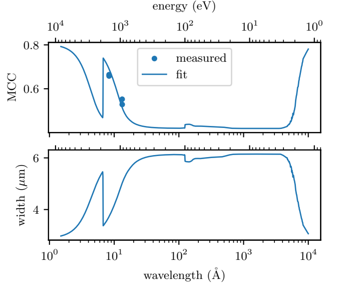
Figure 7. The top panel plots the MCC measured by R. A. Stern et al. (2004) and the fit of our model. The bottom panel shows the corresponding standard deviation of the charge diffusion kernel for the J. Heymes et al. (2020) sensor.
