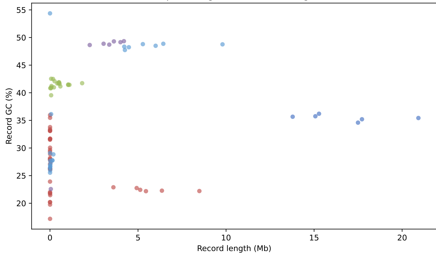
GC percentage versus record length
