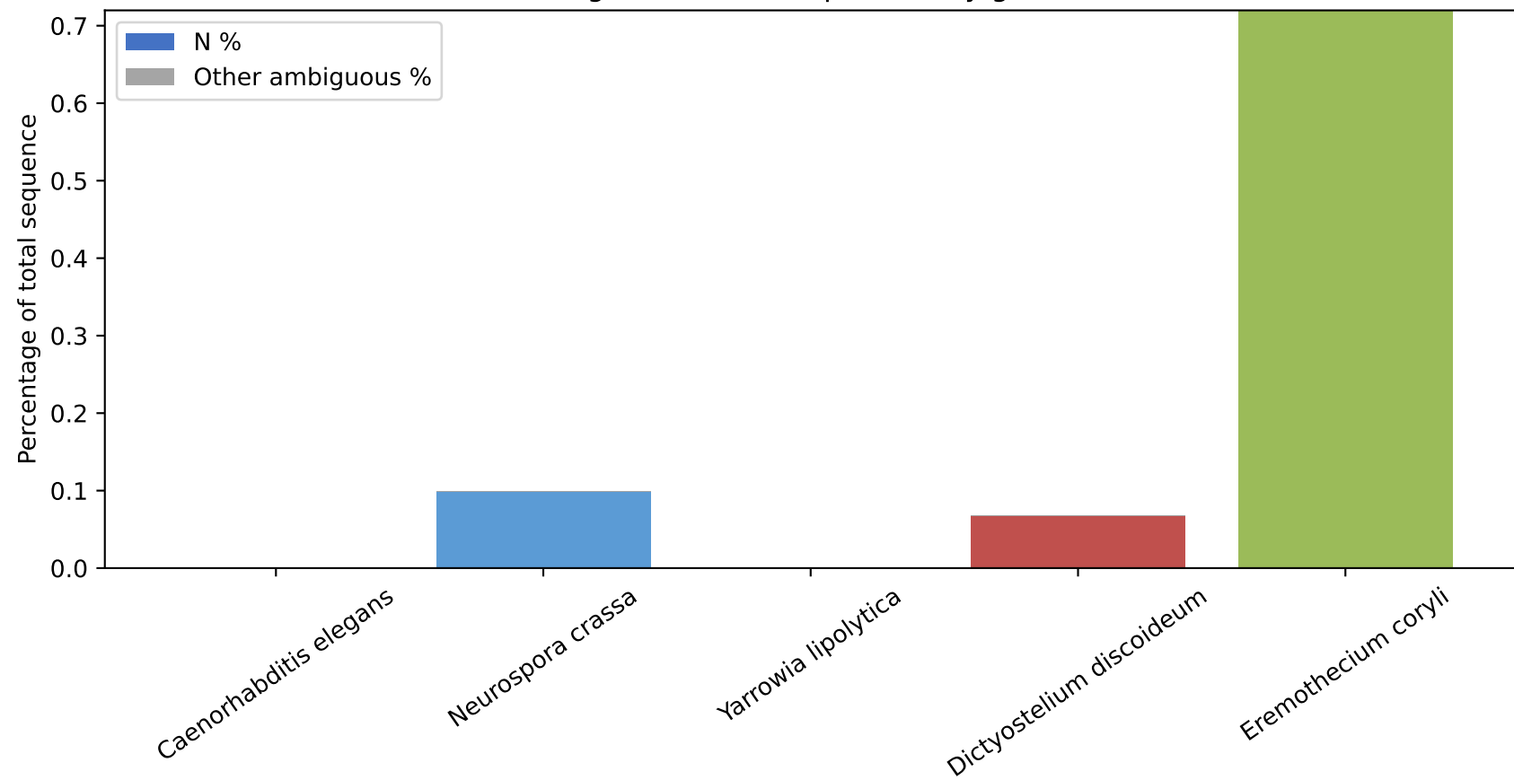
Ambiguous-base composition by genome
