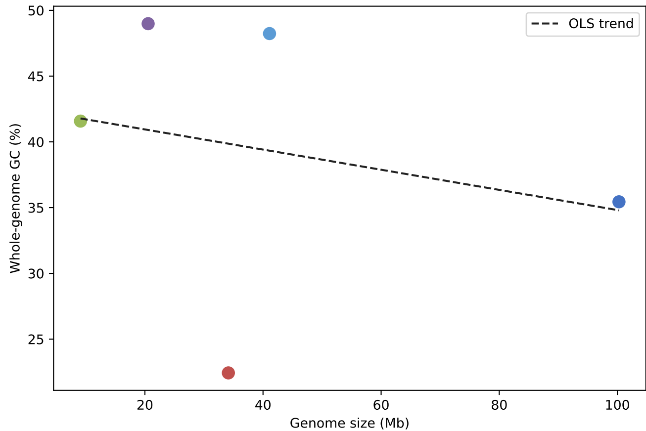
Genome size versus GC with fitted trend
