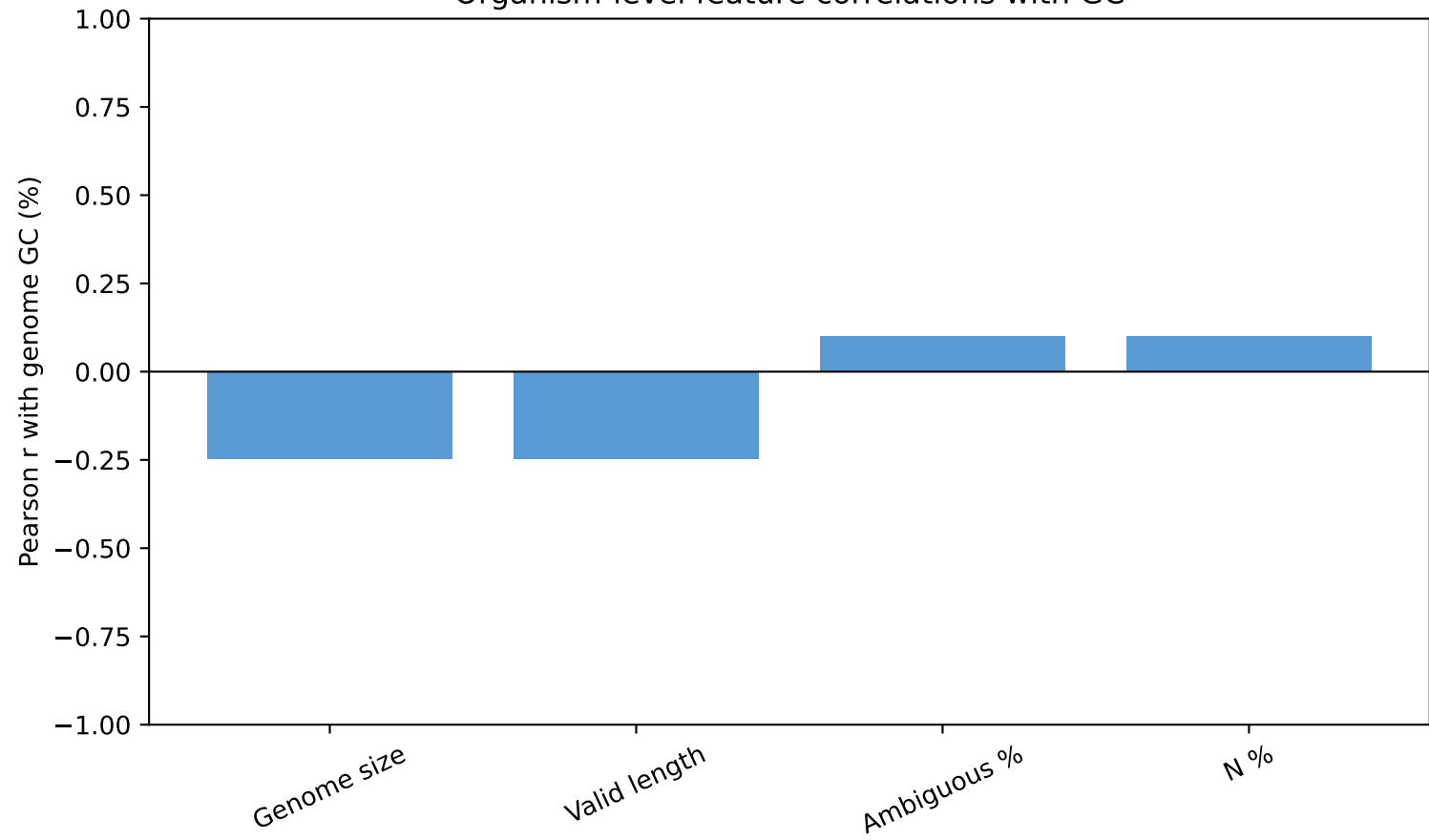
Organism-level feature correlations with GC
