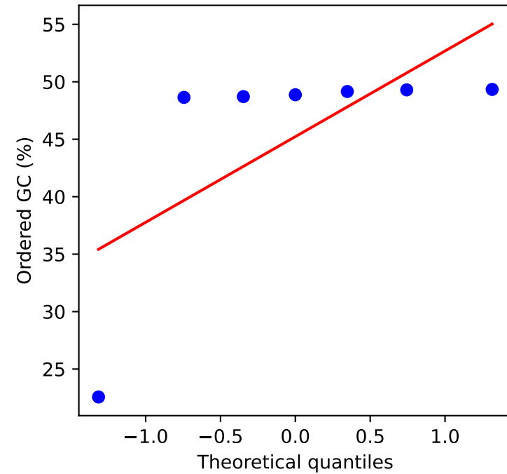
Yarrowia lipolytica
