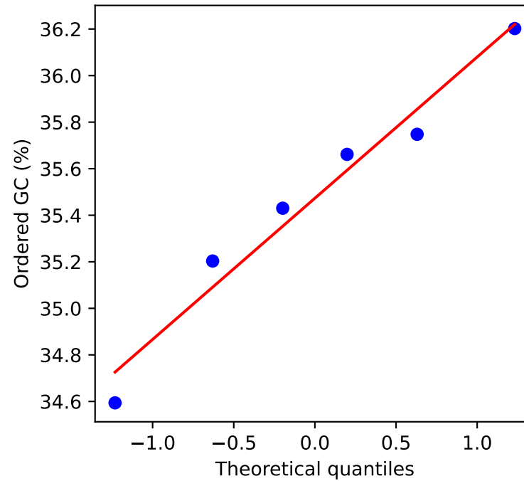
Caenorhabditis elegans
