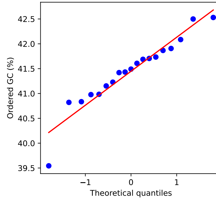
Eremothecium coryli
