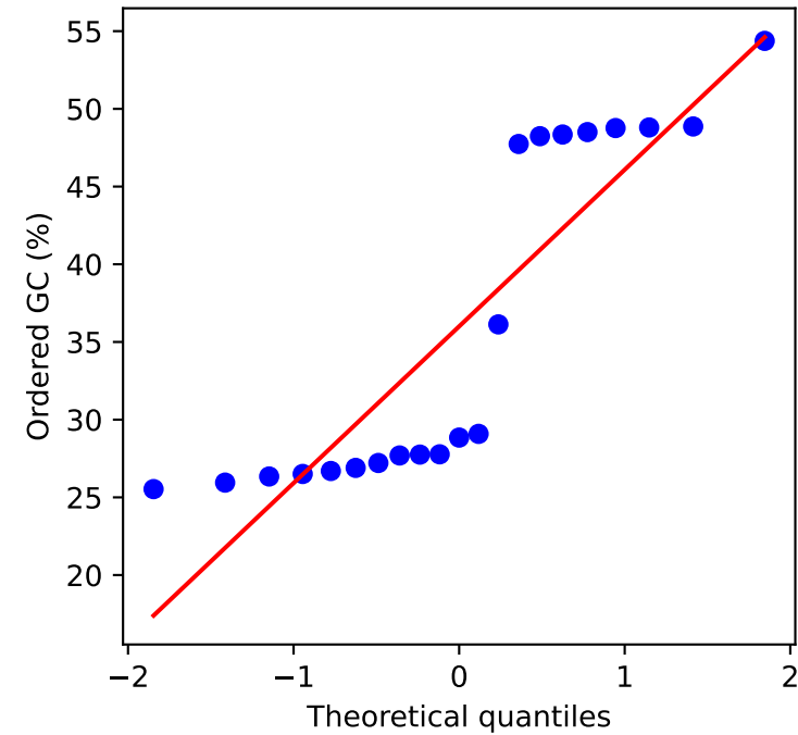
Neurospora crassa
