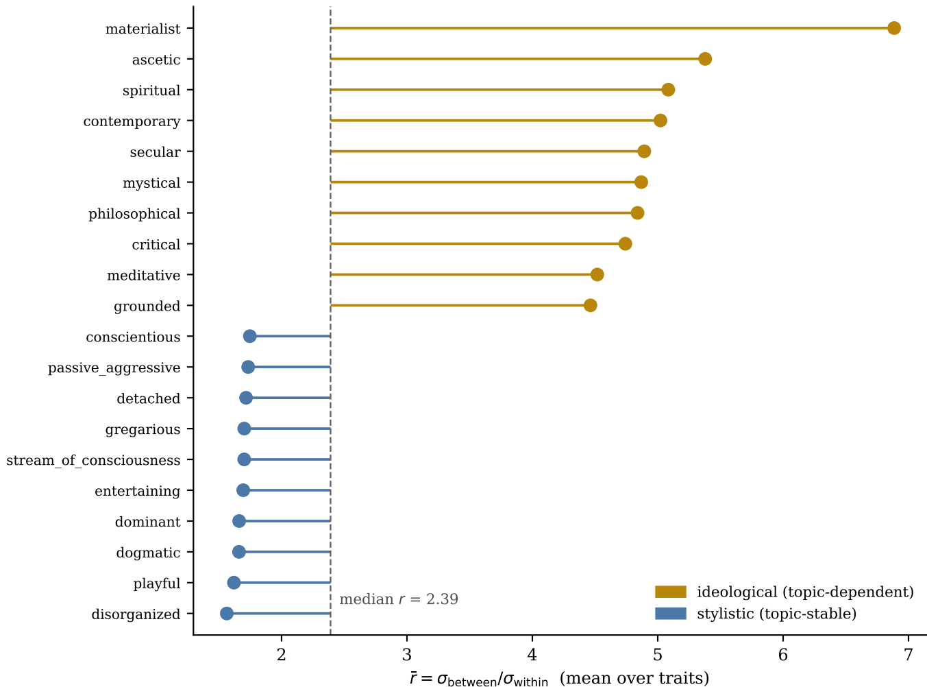
Topic-dependence by axis (NQ): ideological axes vary most across topics
