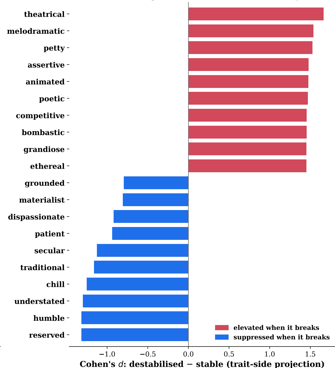
(b) Persona signature of a destabilised response
