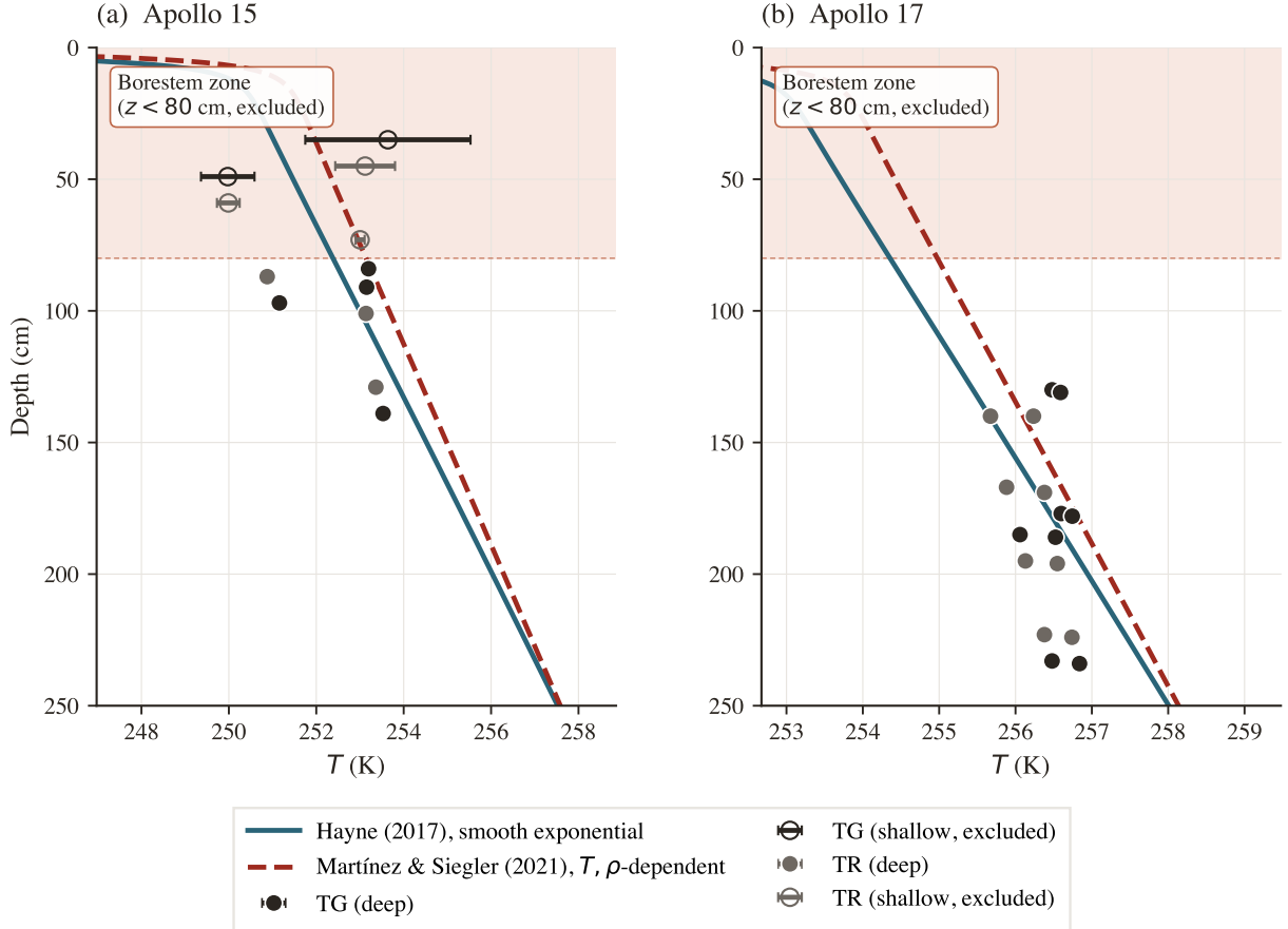
Figure 5. Annual-mean subsurface temperature \langle T(z) \rangle for the two published conductivity models at their nominal (un-retrieved) parameters, Hayne et al. (2017) smooth exponential at the global K_d = 3.4 \text{ mW}/(\text{m K}) (solid), and the Martínez and Siegler (2021) temperature- and density-dependent K(T, \rho) forward (dashed), against the Apollo HFE stability-window means. Markers are coded by sensor type (charcoal = TG, grey = TR); horizontal bars are the within-window standard deviation. The shaded band is the borestem-contaminated zone ( z < 80 \text{ cm} ), excluded from the RMSE.
