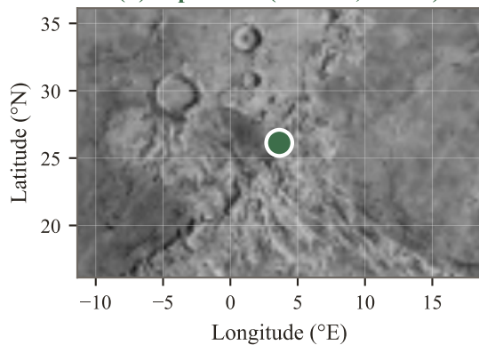
(b) Apollo 15 ( 26.1^{\circ} N, 3.6^{\circ} E)
