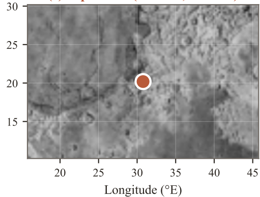
(c) Apollo 17 ( 20.2^{\circ} N, 30.8^{\circ} E)
