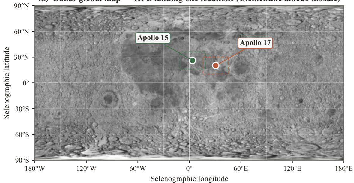
(a) Lunar global map — HFE landing-site locations (Clementine albedo mosaic)
