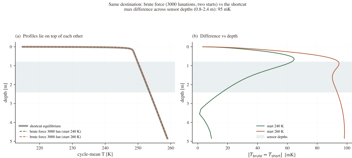
Figure 7: Fully converged brute force from 240 K and 260 K (dashed) overlaid on the shortcut (solid). The profiles are indistinguishable; the residual (right, tens of mK) is just brute force finishing its slow descent.
