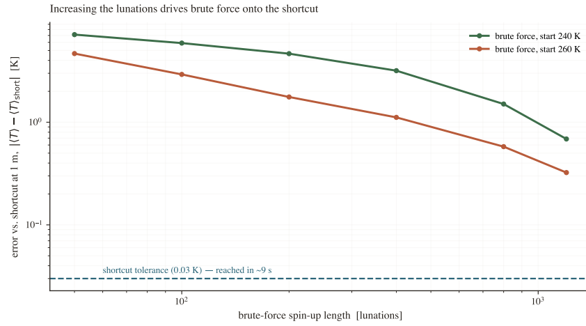
Figure 6: The “increasing-lunations” graph. Brute-force error (vs. the shortcut, at 1 m) falls steadily as the spin-up lengthens, heading for the shortcut’s certified tolerance (dashed). Two different starting temperatures converge to the same place — evidence that the two methods share one solution.
