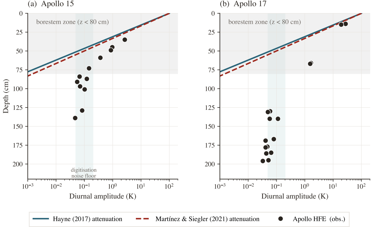
Figure 4. Diurnal amplitude (half-range of the local-solar-time-folded median temperature estimated as \sqrt{2} \times the within-stability-window standard deviation, the half-range of a sinusoidal signal) versus sensor depth at both Apollo sites. Black markers: observed; solid teal: Hayne et al. (2017) regolith attenuation; dashed red: Martínez and Siegler (2021) attenuation, both evaluated at T = 250 K with the published deep-regolith meter-scale regolith density of 1800 \text{ kg m}^{-3} and c_p(250 \text{ K}) \approx 670 \text{ J kg}^{-1} \text{ K}^{-1} , the Hayne form including its radiative conductivity term. The two model curves differ by \sim 10\% in predicted skin depth and are visually indistinguishable on the log axis at all relevant depths. The shaded band is the borestem zone ( z < 80 cm). The order-of-magnitude shallow-sensor excess is the borestem heat-short signature.
