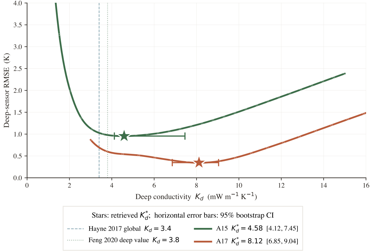
Figure 6. Per-site K_d retrieval under the Hayne et al. (2017) functional form, with all other Hayne et al. (2017) parameters held at their published values. Deep-sensor-Meter-scale-sensor RMSE( K_d ) at each site, extended past the fitting grid so each curve is shown rising again on the high- K_d side: the minima are genuine bracketed bowls, not descending shoulders. Markers: forward-model evaluations; stars: retrieved K_d^* ; shaded band: 95% bootstrap CI; horizontal error bars: 95% bootstrap CI. Dashed vertical: Hayne et al. (2017) global K_d = 3.4 ; dotted: the Feng et al. (2020) deep value K_d = 3.8 .
