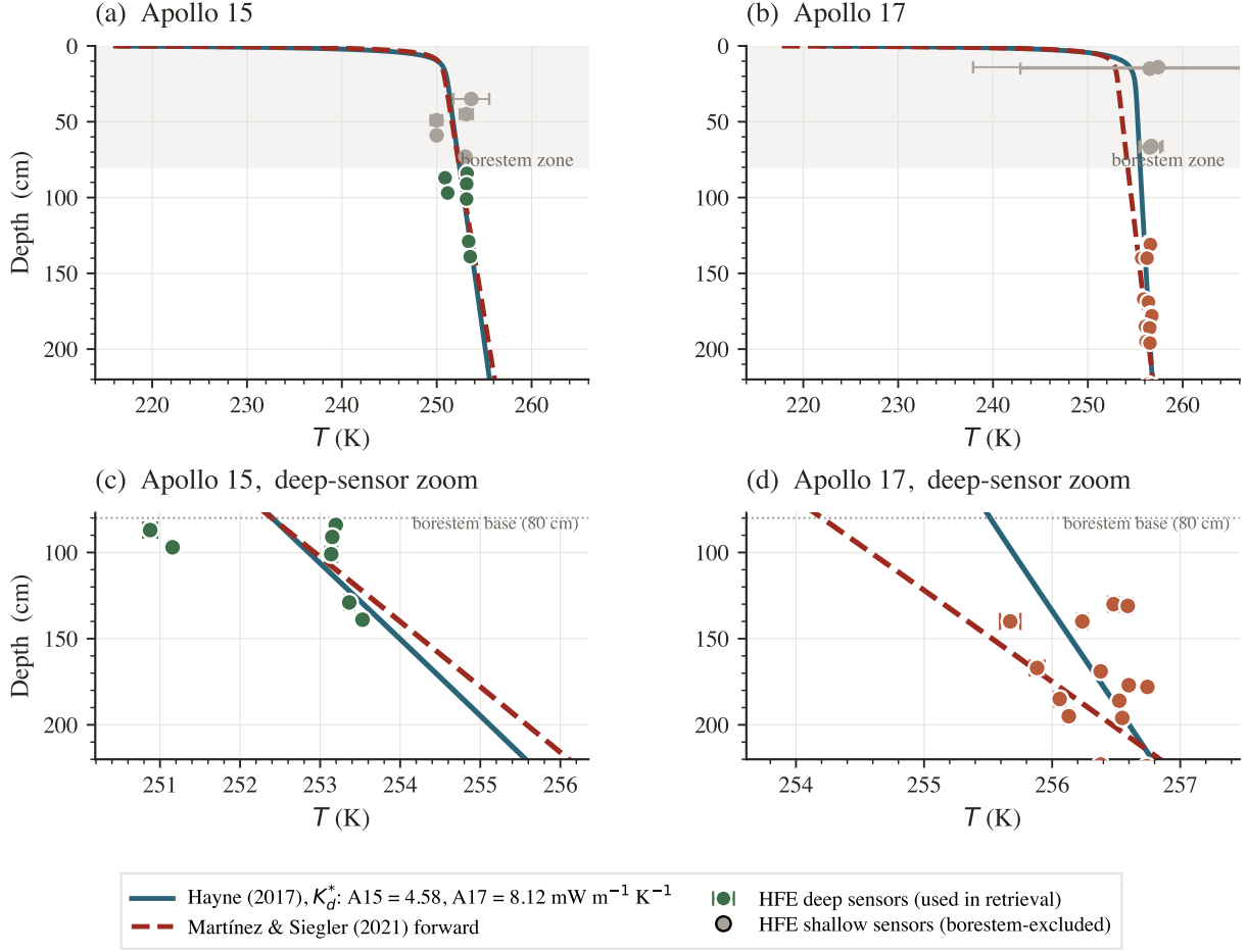
Figure 8. Annual-mean T(z) at the two sites under the two conductivity models, against the Apollo HFE deep-meter-scale sensors. Solid teal: Hayne et al. (2017) at the per-site retrieved K_d^* ; dashed red: Martínez and Siegler (2021) forward (no fitted knob). Top: full profile; bottom: deep-sensor-meter-scale-sensor zoom. Coloured markers: HFE deep-meter-scale sensors (used in retrieval); grey markers: borestem-affected shallow sensors (excluded).
