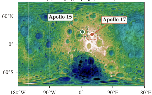
(a) Topography (LOLA)
