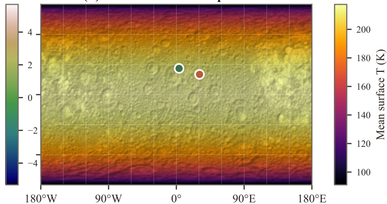
(b) Mean surface temperature
