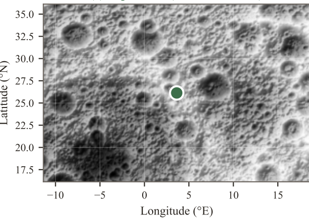
(c) Apollo 15 ( 26.1^{\circ} N, 3.6^{\circ} E)
