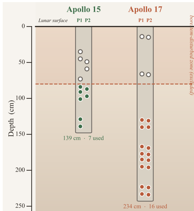
(a) Apollo HFE probe emplacement
