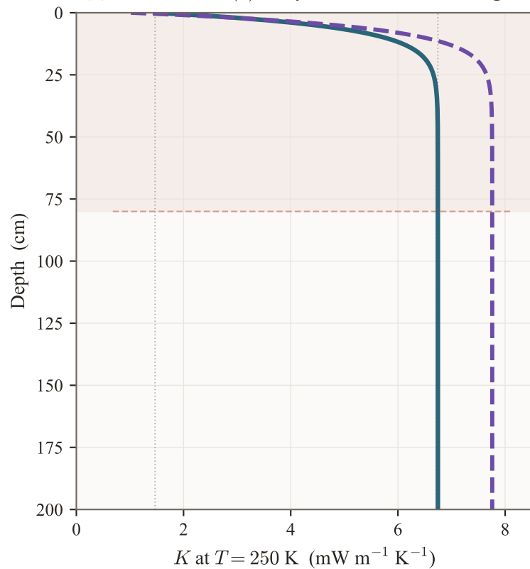
(b) Published K(z) : Hayne vs Martínez & Siegler
