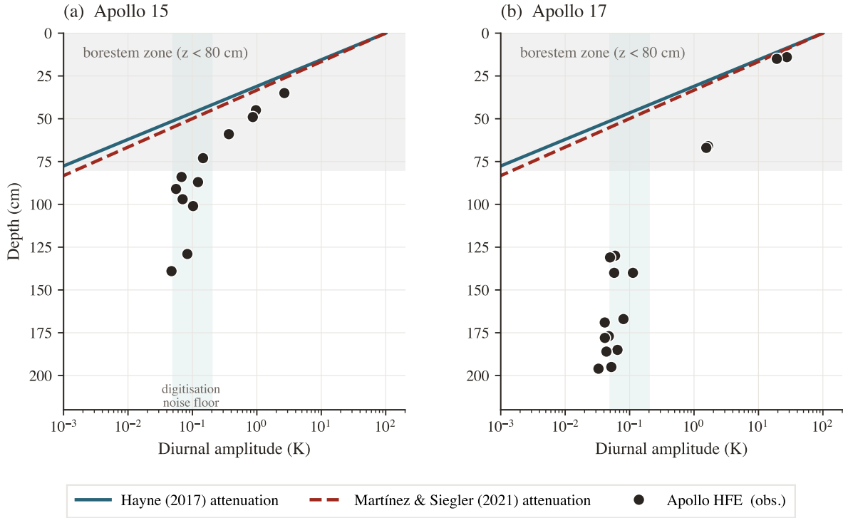
Figure 13. The borestem diagnostic. Black dots: the measured daily temperature wiggle at each sensor. Curves: what physics predicts. Above 80 cm (shaded) the measured wiggle is far larger than physics allows — the fibreglass stem leaking surface heat. Below 80 cm the predicted wiggle is below the record’s noise, so deep sensors carry no usable wiggle, only the steady temperature we want.
