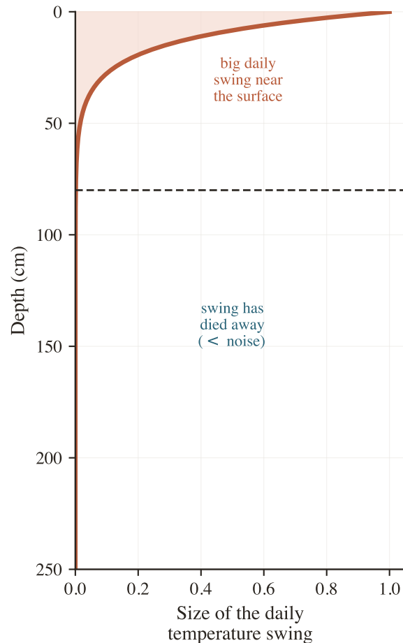
(b) Why deep sensors see a steady temperature
