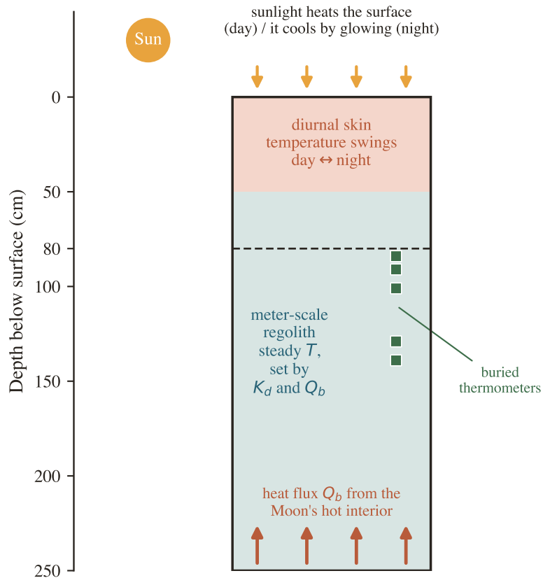
(a) Heat in, heat out, and what is in between
