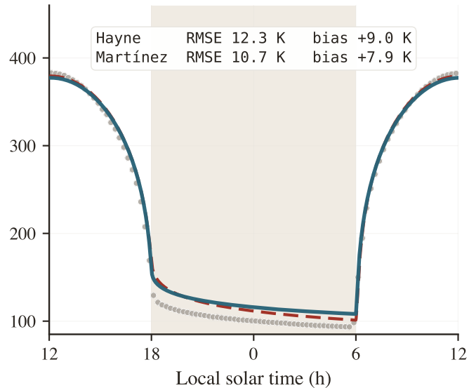
(b) Apollo 17
