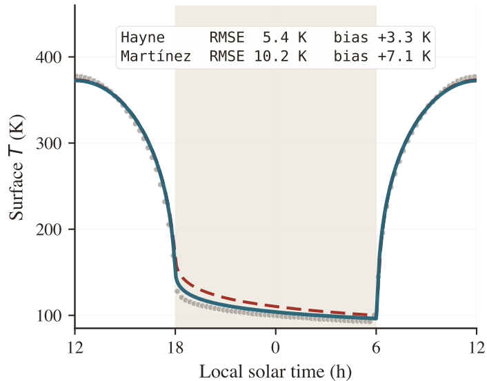
(a) Apollo 15
