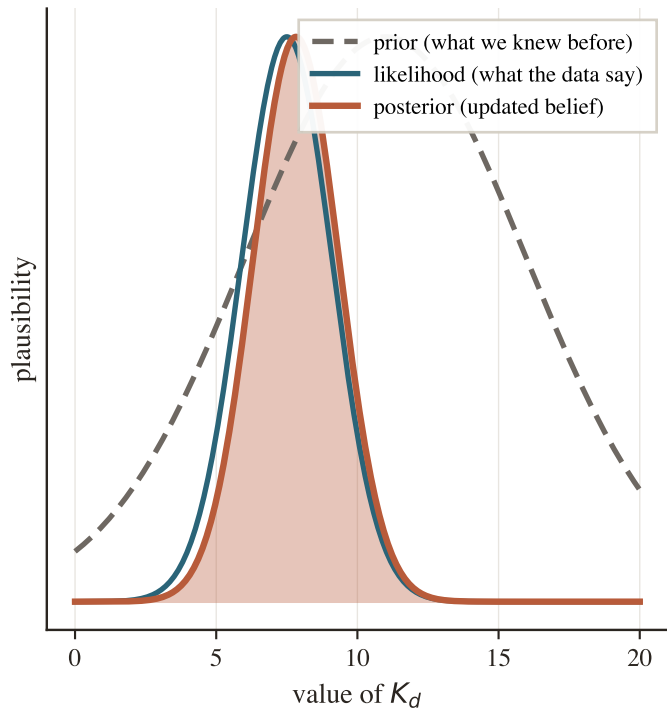
(a) Bayes' rule: update with data
