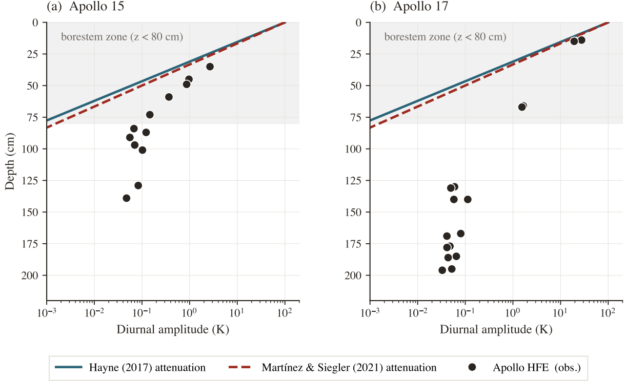
Figure 4. Diurnal amplitude ( half-range-of-the-local-solar-time-folded-median-temperature estimated as \sqrt{2} \times the within-stability-window standard deviation, the half-range of a sinusoidal signal) versus sensor depth at both Apollo sites. Black markers: observed; solid teal: Hayne et al. (2017) regolith attenuation; dashed red: Martínez and Siegler (2021) attenuation, both evaluated at T = 250 K with the published deep-regolith meter-scale regolith density of 1800 \text{ kg m}^{-3} and c_p(250 \text{ K}) \approx 670 \text{ J kg}^{-1} \text{ K}^{-1} , the Hayne form including its radiative conductivity term. The two model curves differ by \sim 10\% in predicted skin depth and are visually indistinguishable on the log axis at all relevant depths. The shaded band is the borestem zone ( z < 80 cm). The order-of-magnitude shallow-sensor excess is the borestem heat-short signature.
