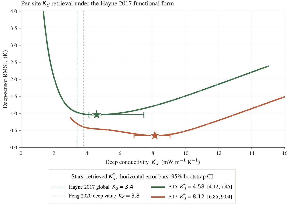
Figure 6. Per-site K_d retrieval under the Hayne et al. (2017) functional form, with all other Hayne et al. (2017) parameters held at their published values. Deep-sensor-Meter-scale-sensor RMSE( K_d ) at each site, extended past the fitting grid so each curve is shown rising again on the high- K_d side: the minima are genuine bracketed bowls, not descending shoulders. Markers: forward-model evaluations; stars: retrieved K_d^* ; shaded band: 95% bootstrap CI; horizontal error bars: 95% bootstrap CI. Dashed vertical: Hayne et al. (2017) global K_d = 3.4 ; dotted: the Feng et al. (2020) deep value K_d = 3.8 .
