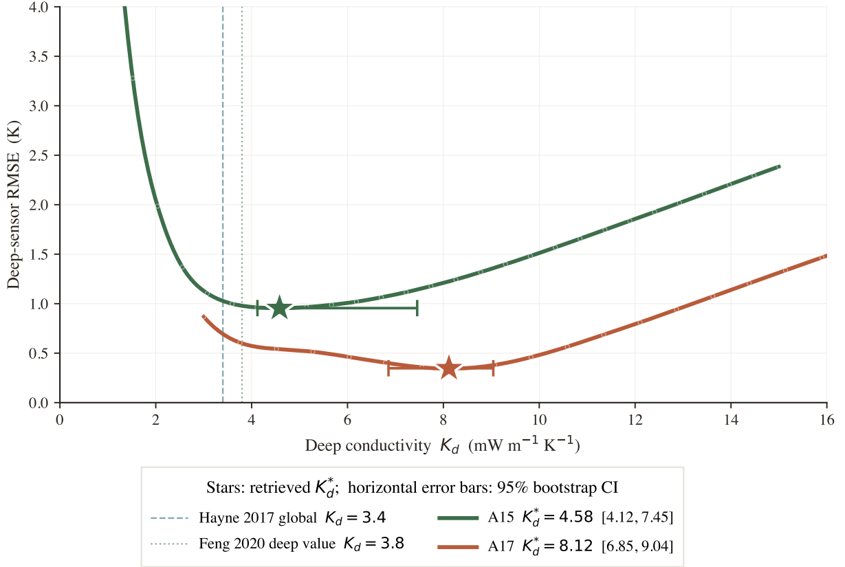
Figure 6. Per-site K_d retrieval under the Hayne et al. (2017) functional form, with all other Hayne et al. (2017) parameters held at their published values. Deep-sensor RMSE( K_d ) at each site, extended past the fitting grid so each curve is shown rising again on the high- K_d side: the minima are genuine bracketed bowls, not descending shoulders. Markers: forward-model evaluations; stars: retrieved K_d^* ; shaded band: 95% bootstrap CI; horizontal error bars: 95% bootstrap CI. Dashed vertical: Hayne et al. (2017) global K_d = 3.4 ; dotted: the Feng et al. (2020) deep value K_d = 3.8 .
