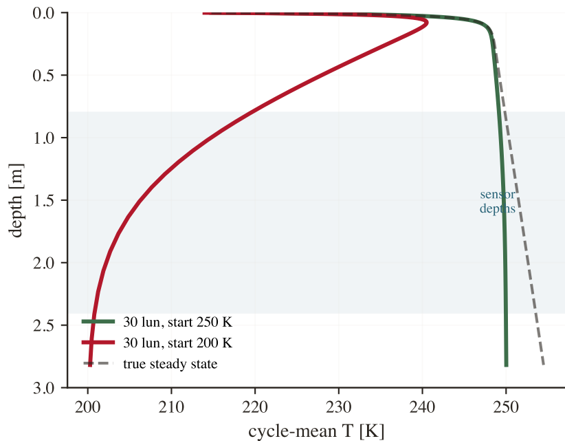
(a) OLD method: 30 lunations Two starts give different answers (gap \approx 40 K at sensors)
