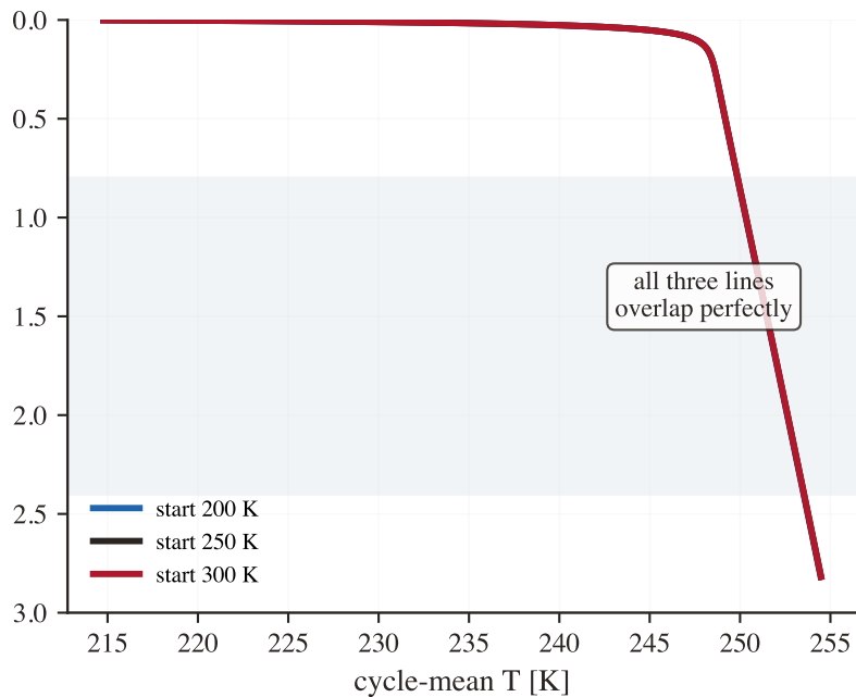
(b) NEW method: three starts All three land on the same profile
