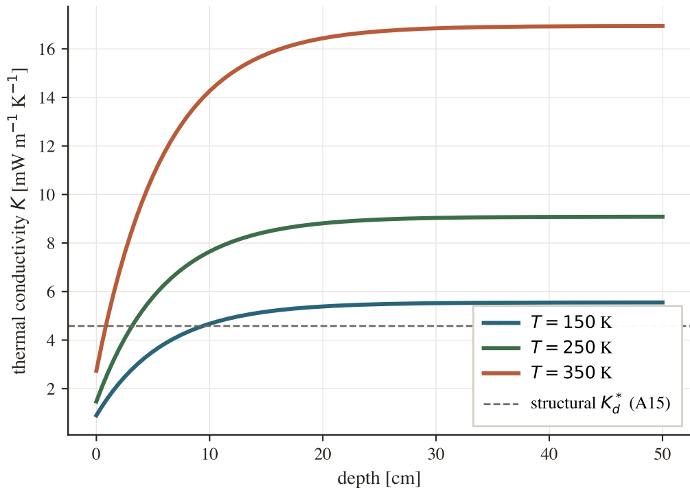
Conductivity rises with depth and temperature
