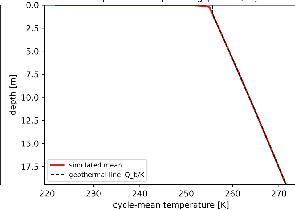
deep MEAN keeps rising (0.85 K/m)
