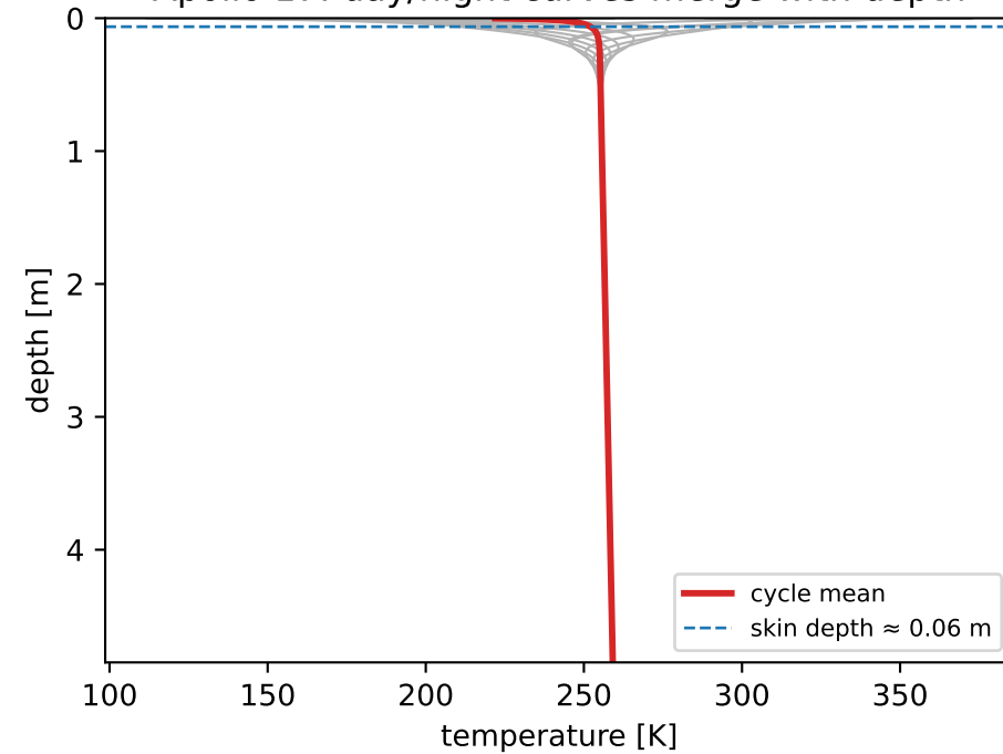
Apollo 17: day/night curves merge with depth
