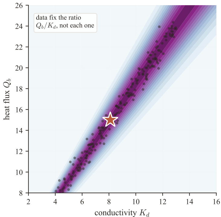
(b) Why one borehole can't separate them
