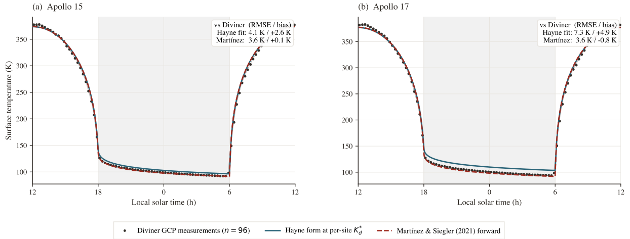
Figure 11. Surface- T closure against the Williams et al. (2017) Diviner GCP diurnal composite. The orbiter measurements (dark edged markers, n = 96 local-solar-time bins per site, with a faint guide line) are the observational benchmark; the two model curves are overlaid on them. Teal solid: Hayne form at the per-site retrieved K_d^* ; brick-red dashed: Martínez and Siegler (2021) form at published coefficients (no fitted knob). The local-solar-time axis is shifted so midnight sits at panel centre and noon at the edges; the shaded band (LST 18–06) marks the night side. Full-cycle RMSE / mean bias of each model relative to the Diviner data are listed in the inset.
