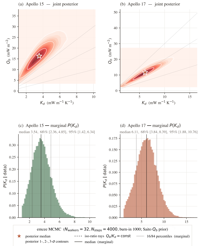
Figure 10: The K_d - Q_b trade-off. Because the deep gradient is Q_b/K , the two are degenerate along a diagonal; the retrieved K_d is conditional on the assumed Q_b . The contrast between sites is more robust than either absolute value.
