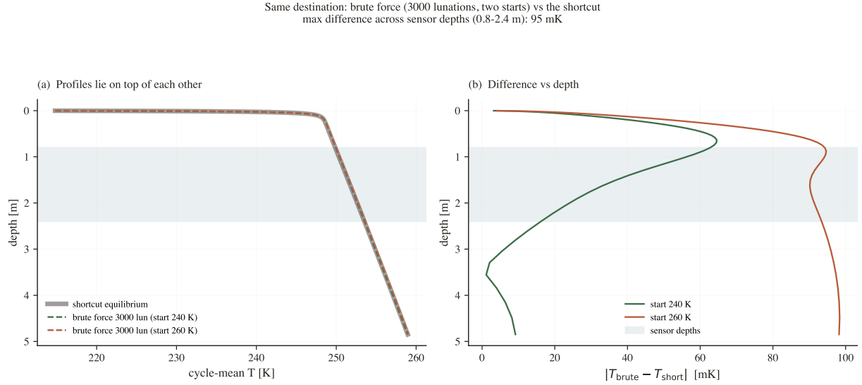
Figure 8: Fully converged brute force from 240 K and 260 K (dashed) overlaid on the shortcut (solid). The profiles are indistinguishable; the residual (right, tens of mK) is just brute force finishing its slow descent.
