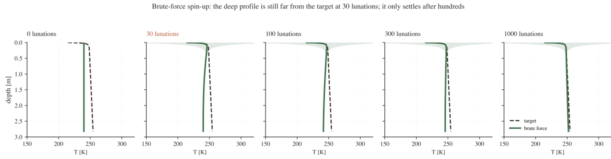
Figure 5: What “brute force” actually is. Snapshots of one spin-up (green = current profile; dashed = the true steady state it is heading for; shaded = the daily temperature swing). At 0 lunations the column is at the flat guess; by 30 lunations only the top has moved while the deep part still sits near the start; it takes hundreds of lunations to reach the target. The “brute-force line” in the other figures is just this green curve once it has finally stopped moving.
