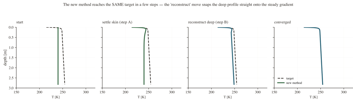
Figure 6: The new method, step by step (compare Fig. 5). A short spin-up settles the skin (Step A); the reconstruct move then integrates d\langle T \rangle / dz = Q_b / K to snap the deep profile onto the steady gradient (Step B); a dozen short rounds refine it to the target. It reaches the same profile as brute force in a tiny fraction of the work.
