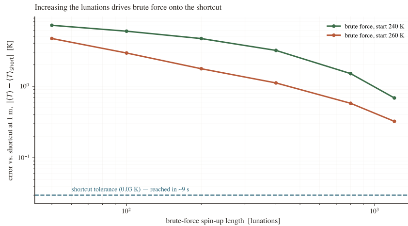
Figure 7: The “increasing-lunations” graph. Brute-force error (vs. the shortcut, at 1 m) falls steadily as the spin-up lengthens, heading for the shortcut’s certified tolerance (dashed). Two different starting temperatures converge to the same place — evidence that the two methods share one solution.
